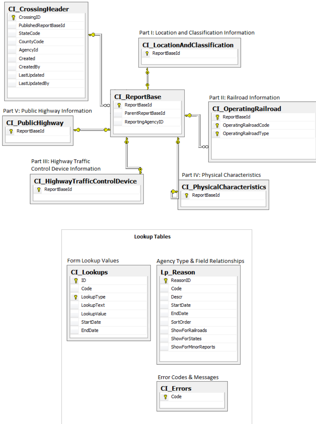
Figure 2-1: GCIS v2.0 Logical Data Model
