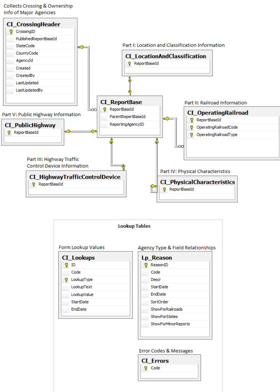
Figure 1 – GCIS v2.0 Logical Data Model
